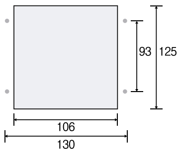
Panel cut
